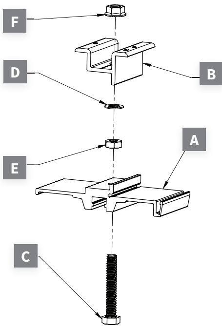
2" Panel Clamp Assembly
