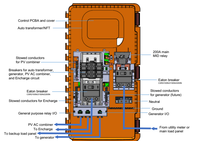
Breaker placement and other connections
