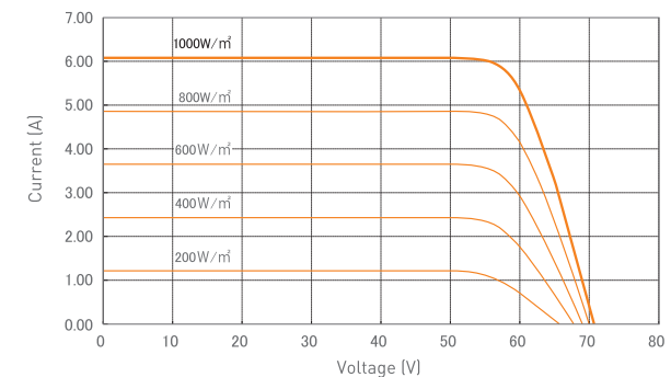
Reference data for model: VBHN330SA17 (Cell temperature: 25°C)
